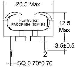
Orthographic view
