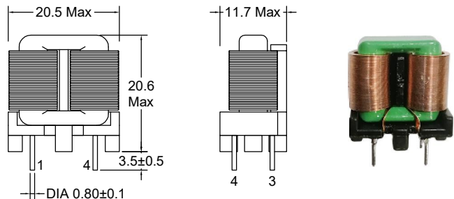
Orthographic view
