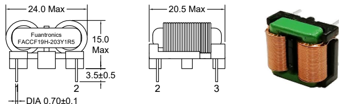
Orthographic view
