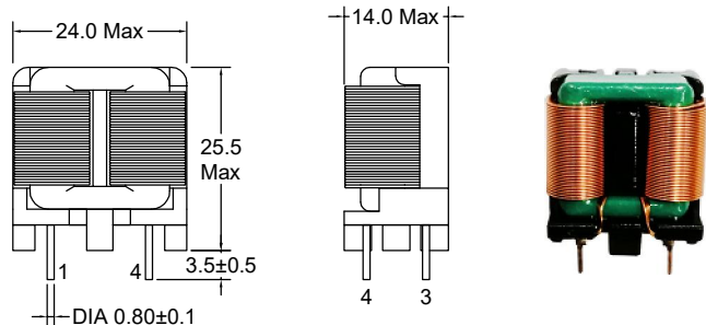
Orthographic view
