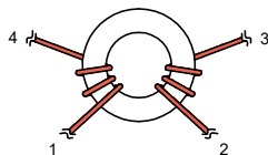
Winding Construction
