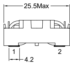
Orthographic view
